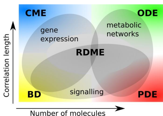
Figure 4: Regimes and models in biochemistry (Dobrzyński et al. 2007). Network models placed in correlation-length versus number-of-molecules space. Abbreviations for (1) models with space: BD—Brownian dynamics, PDE—partial differential equation, RDME—reaction-diffusion master equation, and (2) models without spatial detail: CME—chemical master equation, ODE—ordinary differential equation. ODE and PDE are deterministic models; CME, RDME and BD are stochastic. The correlation length is a measure of the typical length scale at which a system retains its spatial homogeneity.
