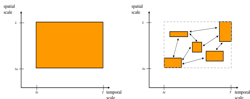
Figure 5: The Scale Separation Map and decomposition of a multiscale system: left, a multi-scale model spanning many temporal and spatial scales; right, the resulting decomposed model, consisting of 5 coupled single scale models.
