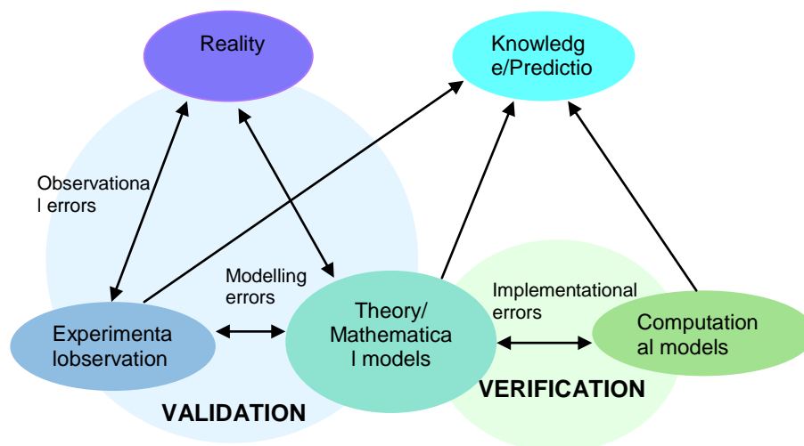
Figure 2. Rigorous modelling needs to address all possible sources of errors to establish their influence on the knowledge based on the experiments, the theoretical model and computational model simulations (adapted from Oden et al. 2010).
